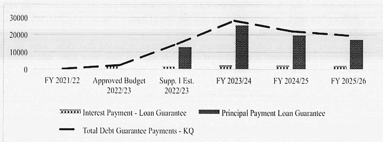
Figure 4: Kenya Airways Guaranteed Debt Payments, (Kshs. Millions)
