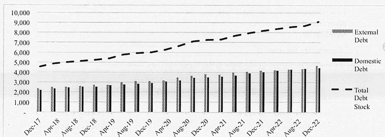
Figure 1: Public Debt Stock, December 2017 – December 2022 (Kshs. Billions)
