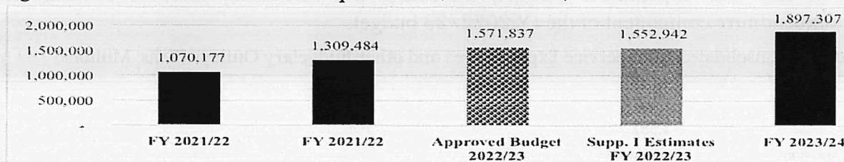
Figure 3: Consolidated Fund Service Expenditures (Kshs. Millions)
