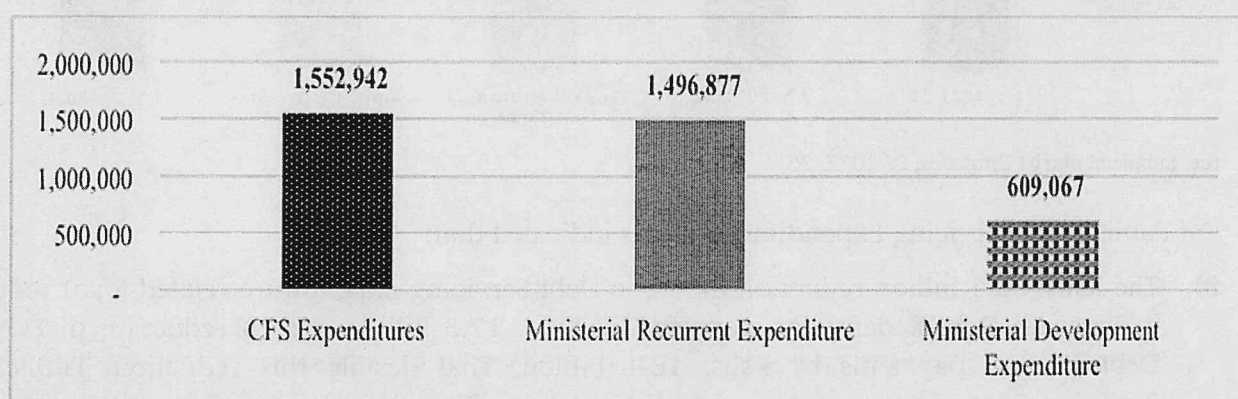
Figure 2: Consolidated Fund Service Expenditures and other Budgetary Outlays (Kshs. Millions)
