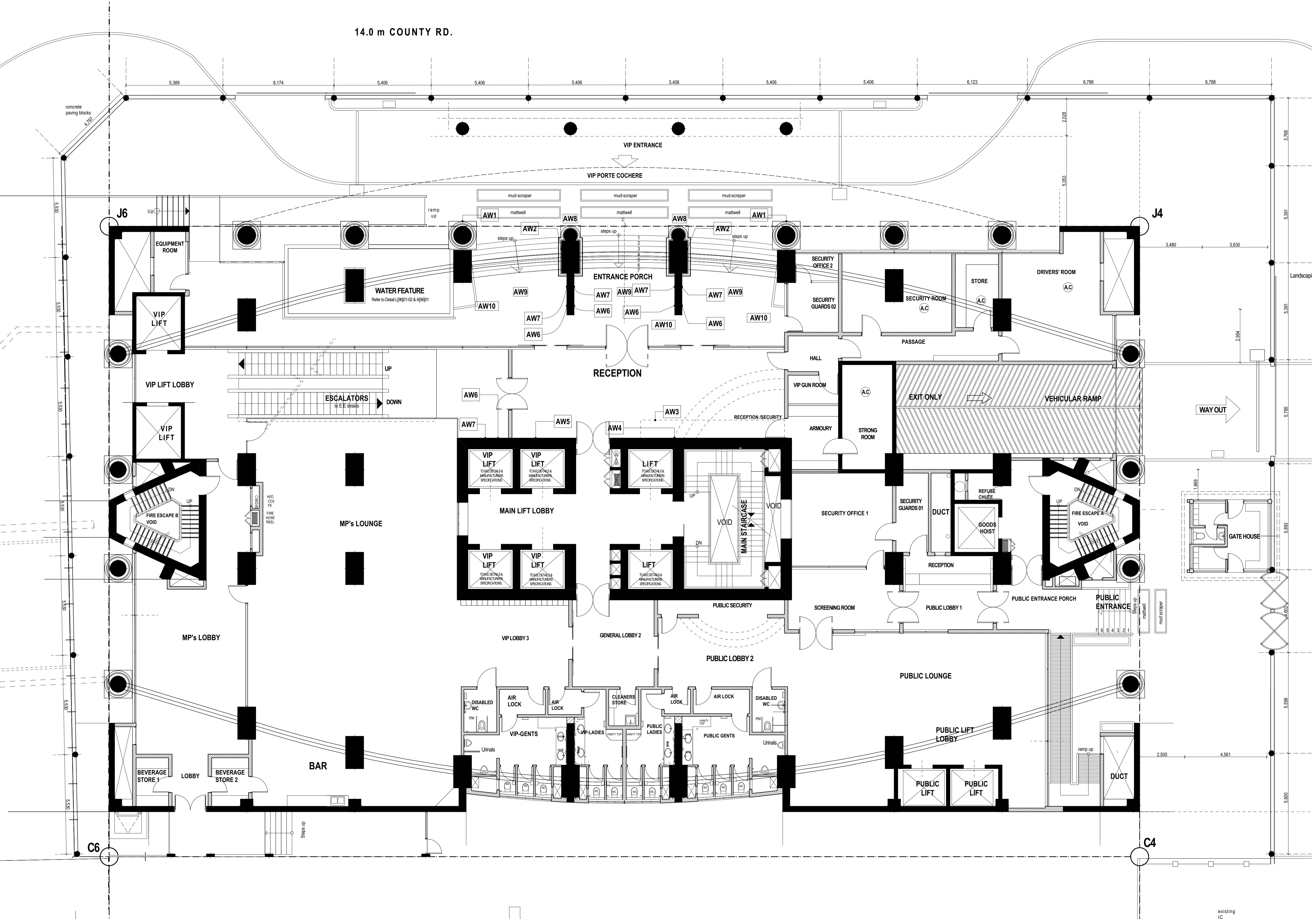
L[--]08 GROUND FLOOR PLAN
